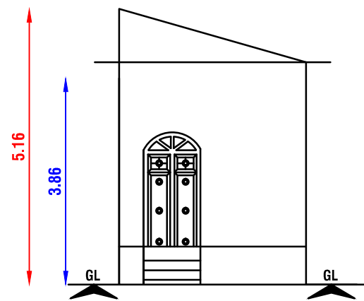
FRONT ELEVATION
