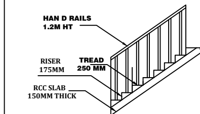
STAIRCASE DETAILS SCALE 1:50
