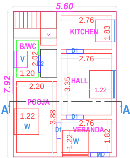
PLAN - FIRST FLOOR ( PROPOSED )
