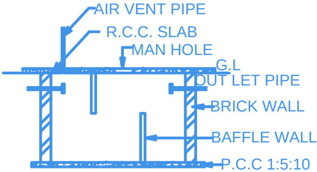
SECTION ON SEP.TANK
