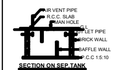
SECTION ON SEPTIC TANK
