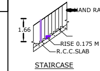
STAIRCASE
