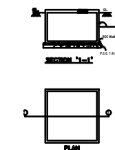
RAIN WATER COLLECTION RAMP DETAIL
