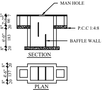
SEPTIC-TANK DETAIL
