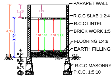
"SECTION "AB"
