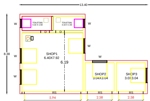
PROPOSED G.FLOOR
