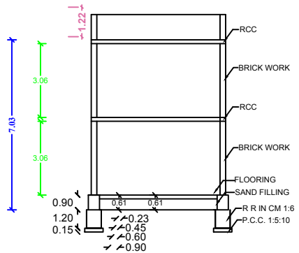
SECTION AB
