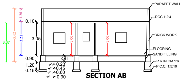
SECTION AB
