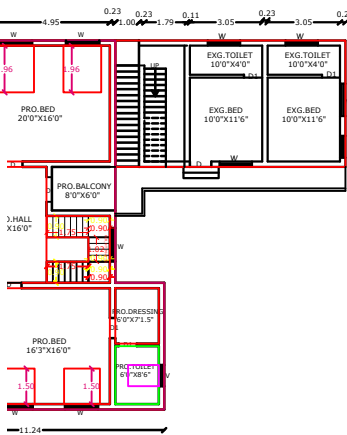
PRO. FIRST FLOOR PLAN
