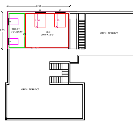
PROPOSED SECOND FLOOR PLAN
