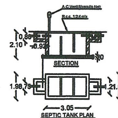
SEPTIC TANK PLAN
