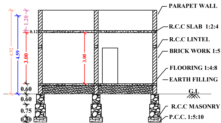
"SECTION "AB"
