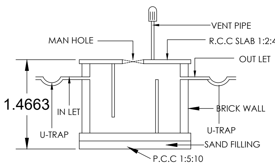
SECTION E,F SEPTIC TANK DETAIL
