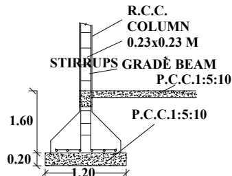
COLUMN DETAIL
