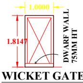
WICKET GATE
