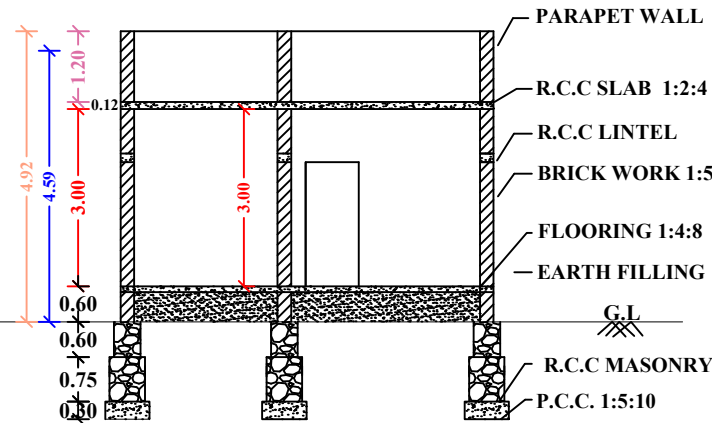
"SECTION "AB"
