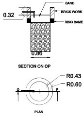
RAIN WATER PIT
