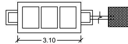
SEPTIC TANK AND TRENCH
