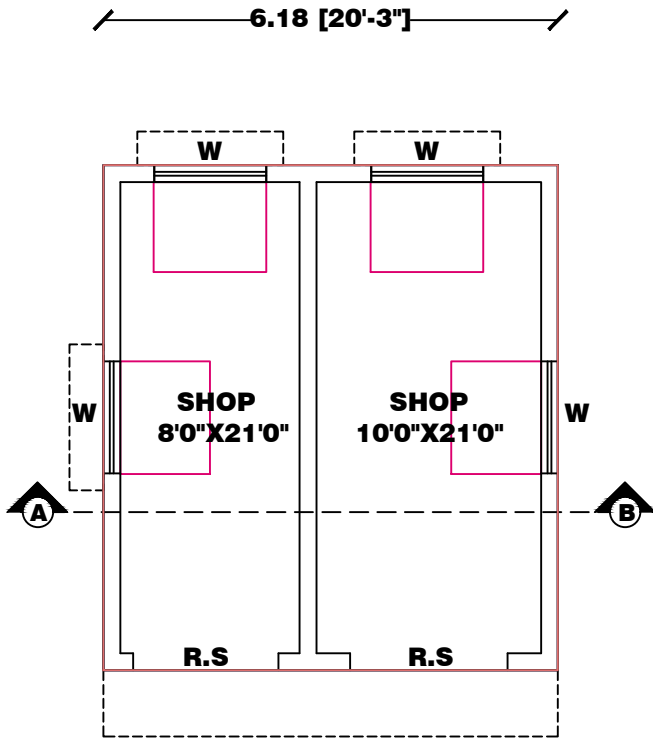
PLAN
