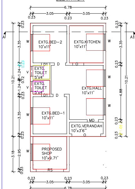
EXISTING/PROPOSED GROUND FLOOR PLAN
