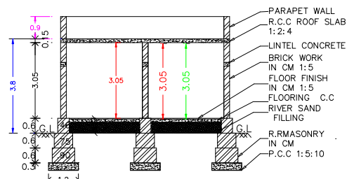
SECTION ON AA1
