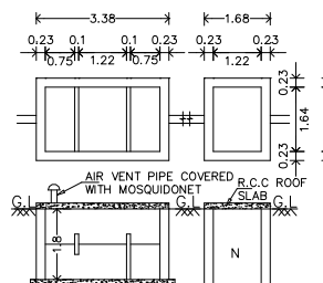
PLAN&SECTION OF SEPTIC TANK 'U' TRAP PROVIDED
