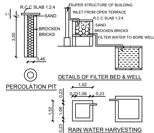
RAIN WATER HARVESTING
