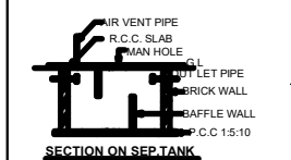
SECTION ON SEPT. TANK
