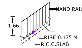
STAIRCASE
