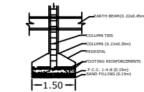
FOUNDATION DETAILS
