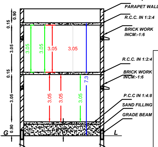
SECTION "AB"
