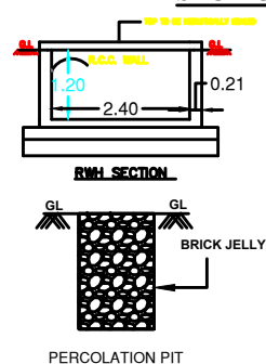
PERCOLATION PIT
