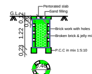
PERCOLATION PIT FOR 30 Sq. m. (Scale:- 1:50)
