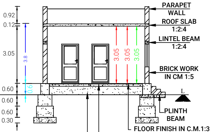
SECTION ON 'AA1'
