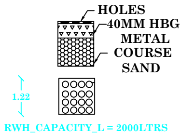
RAIN WATER COLLECTING TANK
