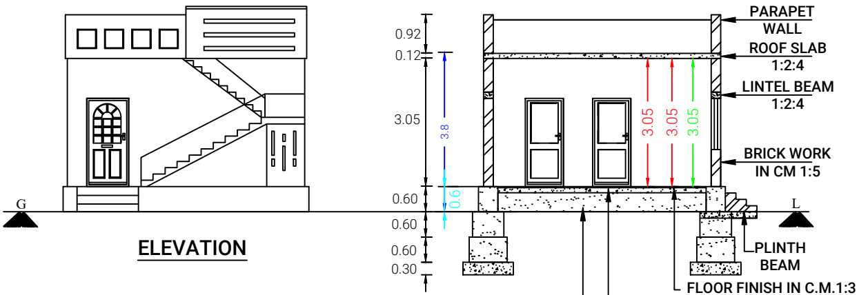
SECTION ON 'AA1'
