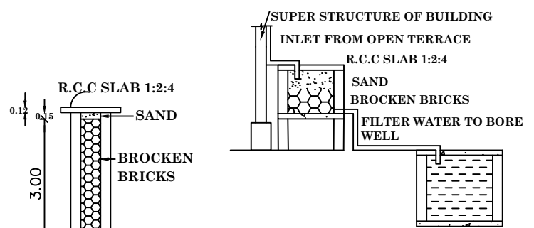
DETAILS OF FILTER BED & WELL
