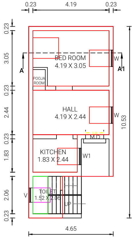
PLAN - GROUND FLOOR (PROPOSED)
