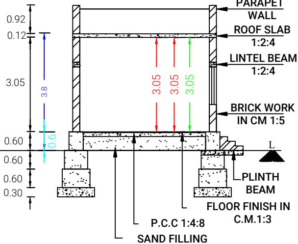
SECTION ON 'AA1'
