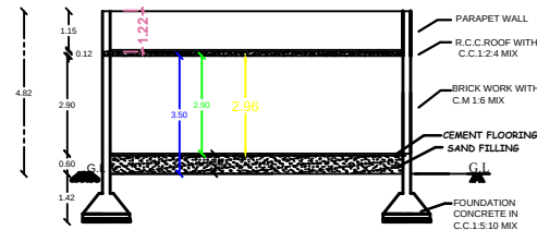
SECTION A & B
