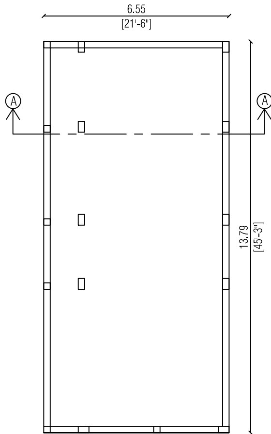
STILT FLOOR PLAN
