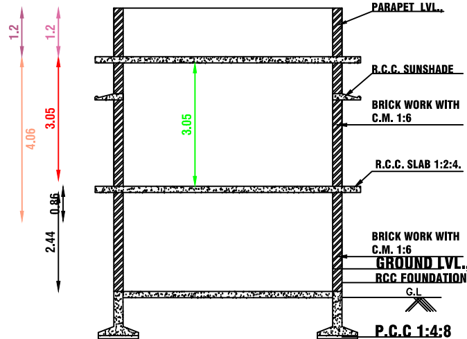
SECTION ON A-A & A'-A'
