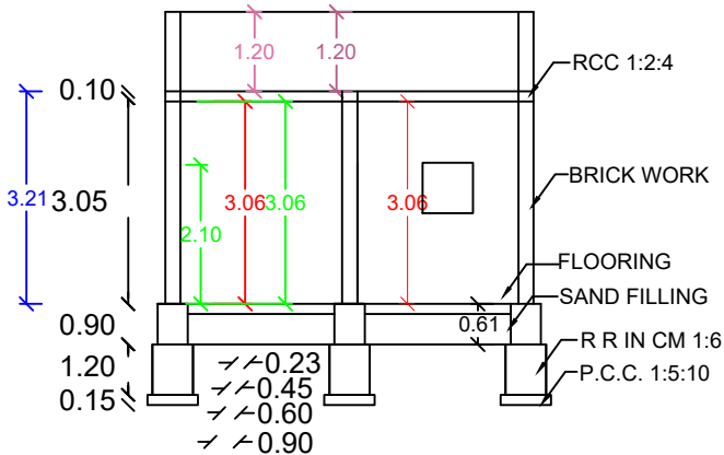
SECTION AB
