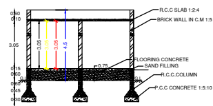
SECTION ON - AA
