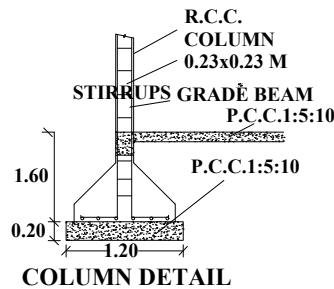
COLUMN DETAIL
