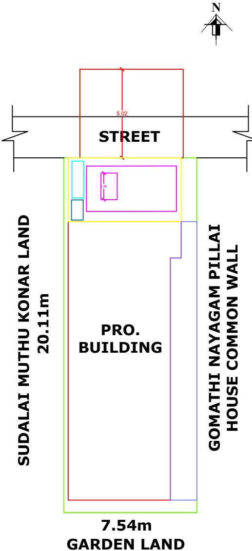
LOCATION PLAN
