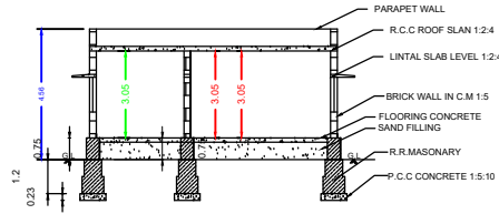
SECTION ON 'AA'
