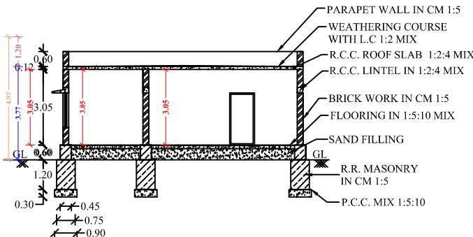
SECTION OF "AB"
