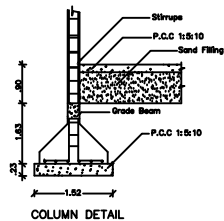
COLUMN DETAIL
