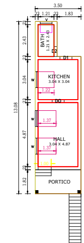
PRO GROUND FLOOR PLAN
