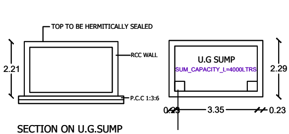
SECTION ON U.G.SUMP
