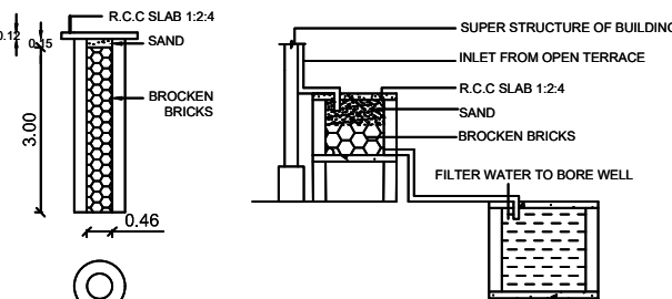
PERCOLATION PIT
