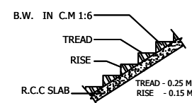
STAIR DETAILS
