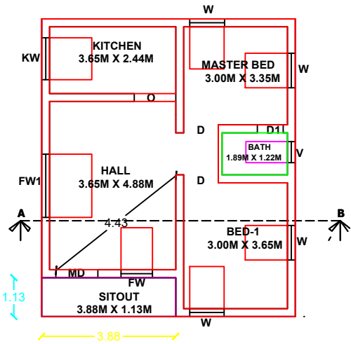
TYPICAL_FLOOR_PLAN=1 GROUND FLOOR PLAN
