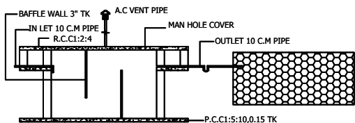
SECTION ON AB 0.46 0.23 0.37 0.23 0.46 3.58 1.53 3.58 SEPTIC TANK AND TRENCH & U TRAP ADOPTED
