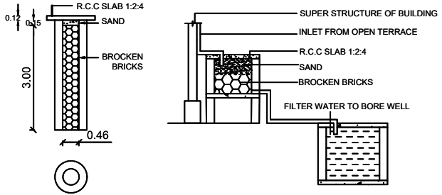
PERCOLATION PIT DETAILS OF FILTER BED & WELL
