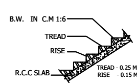
STAIR DETAILS
