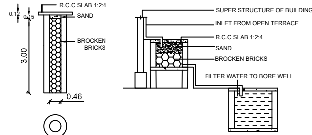
PERCOLATION PIT
