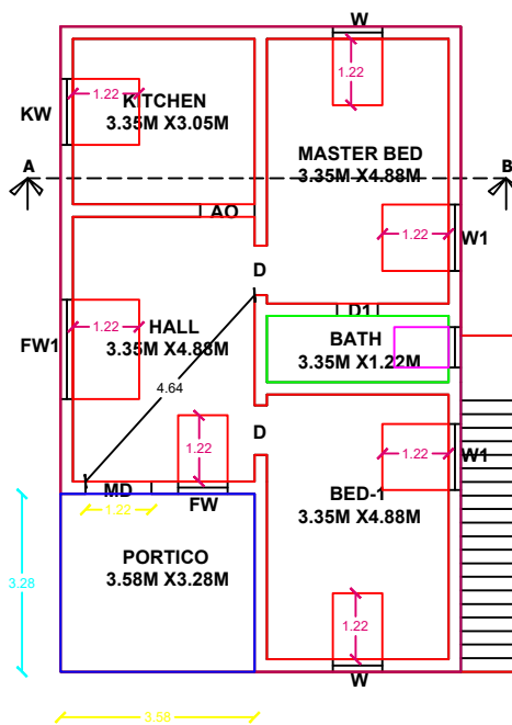
TYPICAL_FLOOR_PLAN=1
