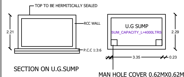
MAN HOLE COVER 0.62MX0.62M
