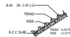
STAIR DETAILS
