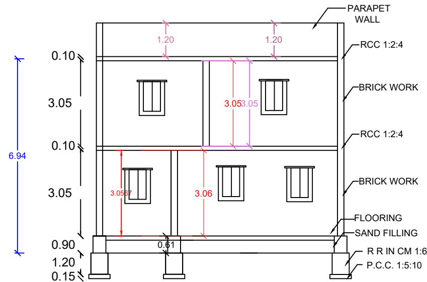
SECTION AB
