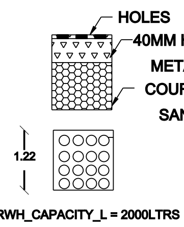
RAIN WATER COLLECTING TANK
