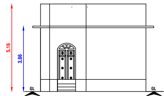
FRONT ELEVATION
