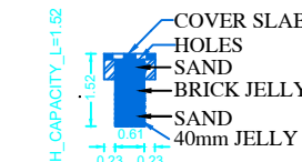
SECTION OF RAIN WATER COLLECTION TANK
