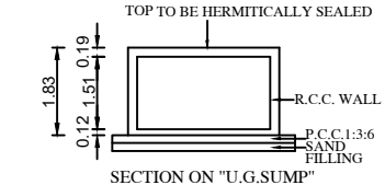
SECTION ON "U.G.SUMP"
