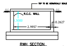
RWH SECTION
