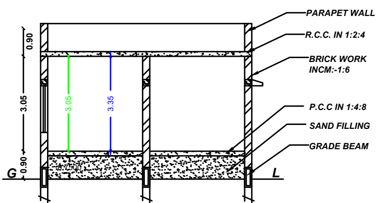
SECTION "AB"
