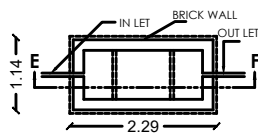
PLAN PLAN OF SEPTIC TANK
