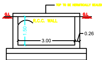
RWH SECTION
