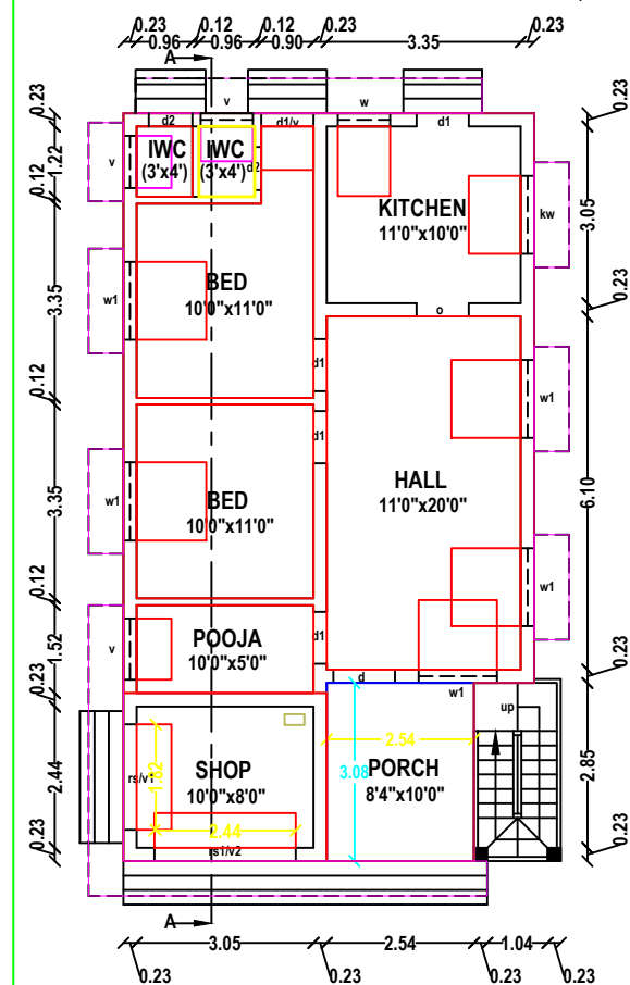
PLAN - GROUND FLOOR RESIDENCE
