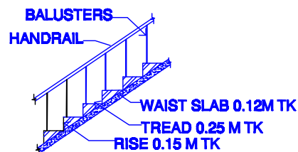
STAIRCASE DETAILS
