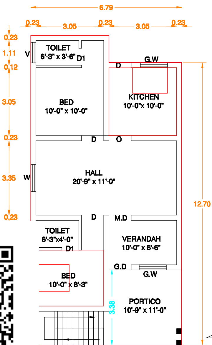
JND FLOOR PLAN
