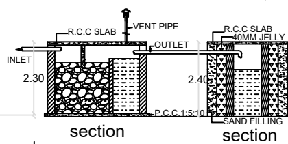
1000 GALLONS CAPACITY SEPTIC TANK (NTS)
