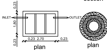
LEACH WELL DETAIL
