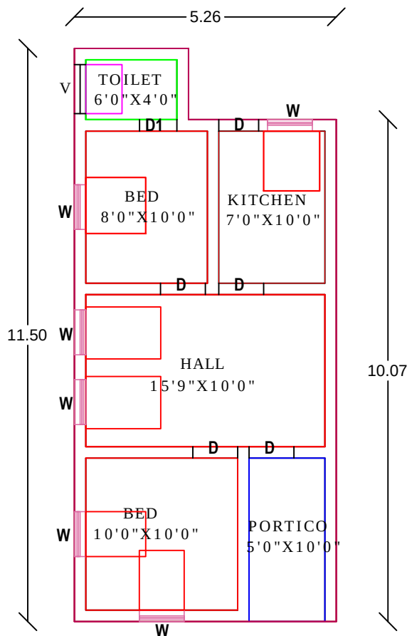
PLAN
