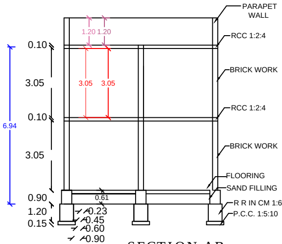
SECTION AB
